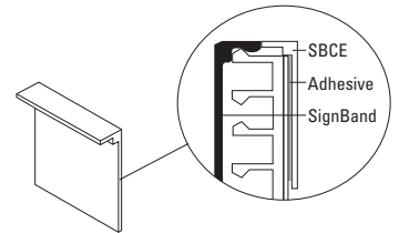
SBCE Optional Top/Bottom Closure Extrusion Side Track System Only
