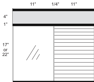
UVR1711(2)-HCL30IS 17"(h) Displays / 14 Bands / 17"x11" ClearLens / 4" Header
