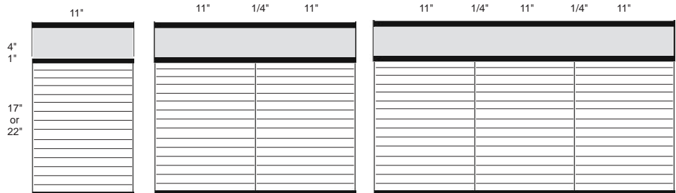
UVR1711-H30IS 17"(h) / 14 Bands / 4" Header
